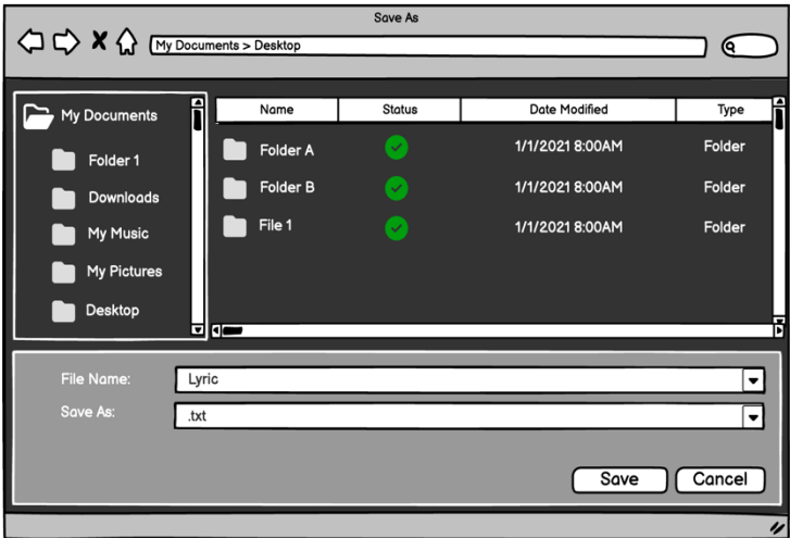
Figure 22 UI05-Save file
