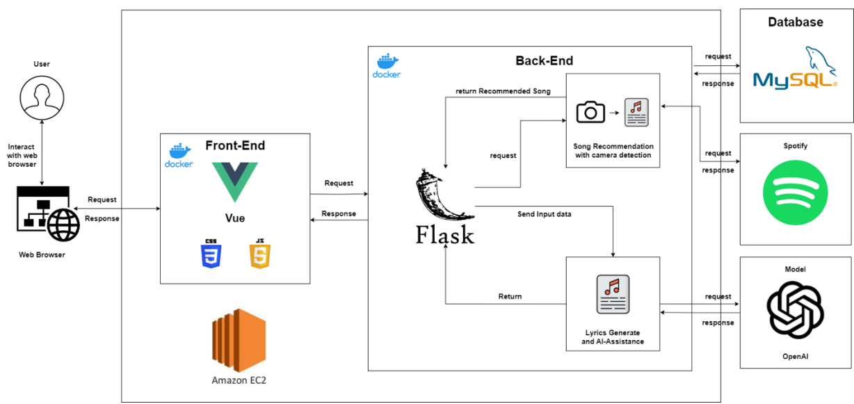
Figure 16 System Architecture
